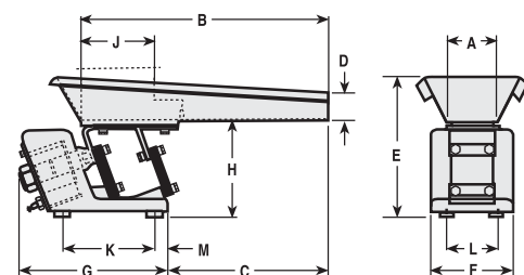
Syntron F-T01 Feeder
