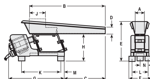
Syntron F-T0 Feeder
