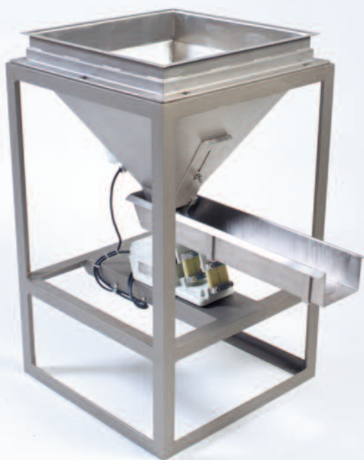
Syntron Volumetric Feeder Machine with customized rectangular hopper.
