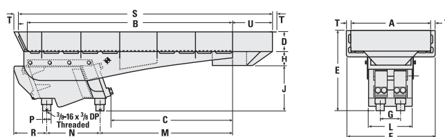
Typical straight type discharge
