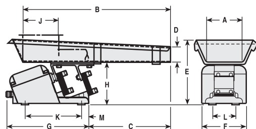
Syntron F-010 Feeder
