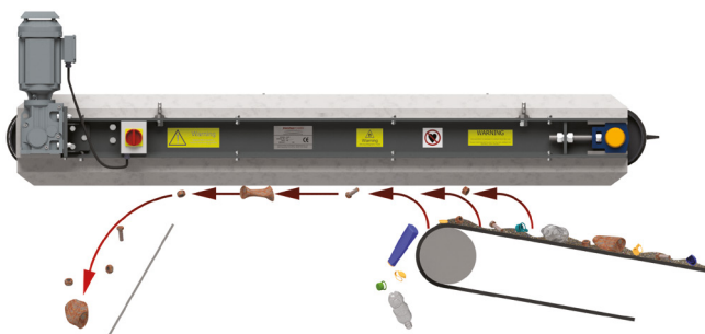
IN-LINE OVERBAND
