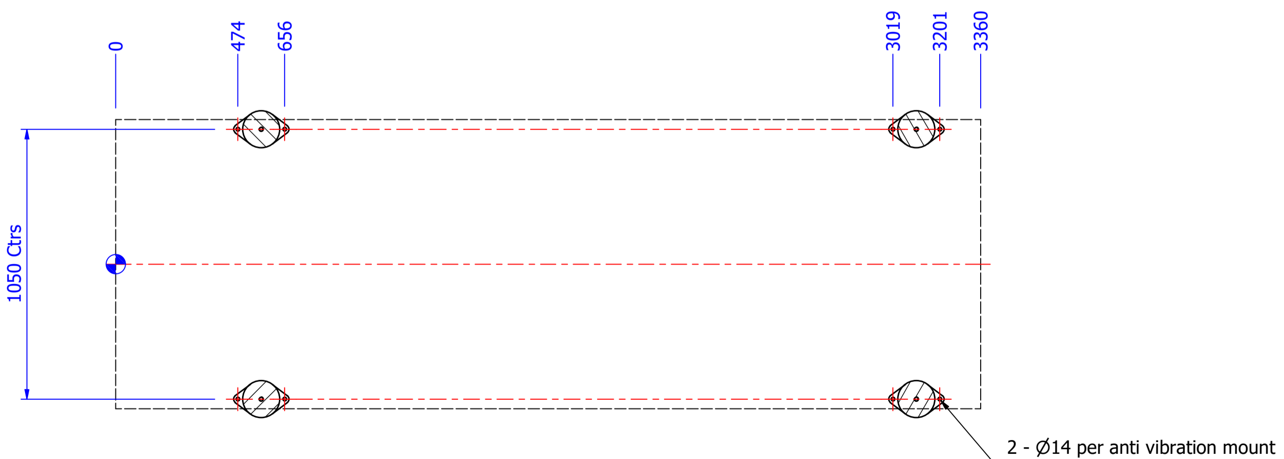
A-A ( 1 : 15 ) Anchor Hole Positions
